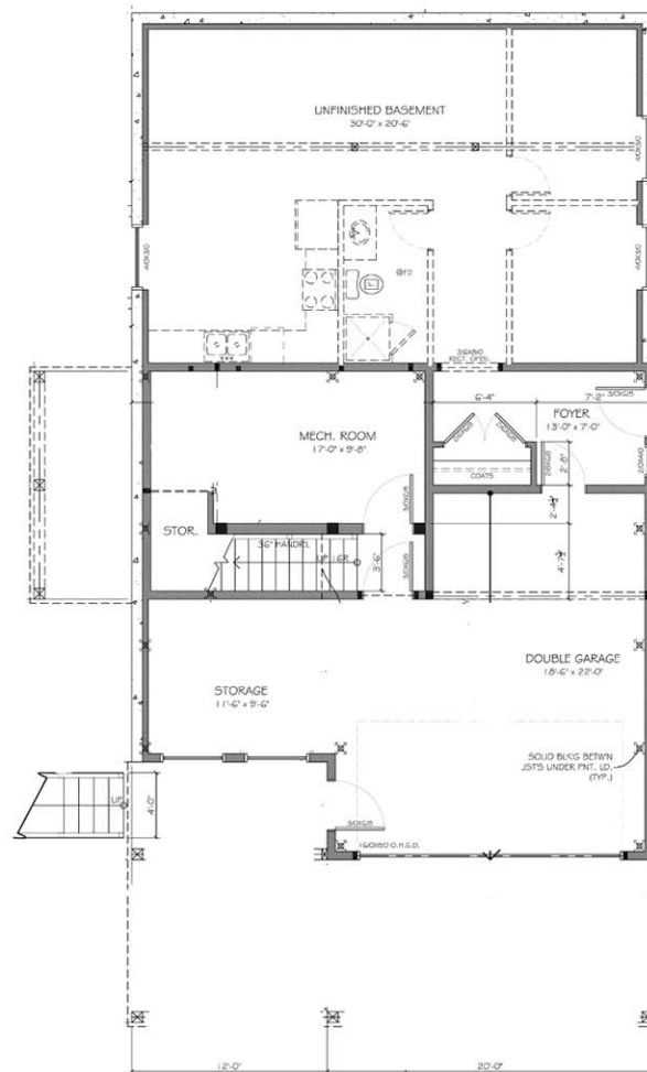
Basement Level Floor Plan
